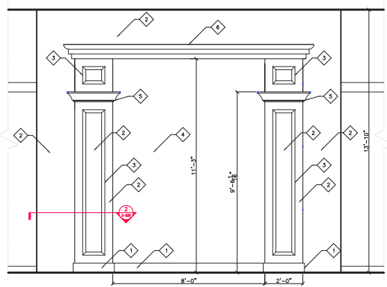
1 TRADITIONAL WALL FEATURE ELEVATION 1/4"=1'-0"
